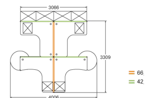
four-person integration
