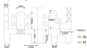
six-person integration
