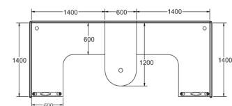
Two-person integration
